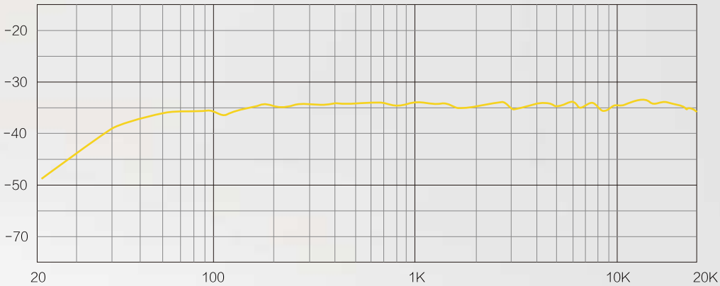
Frequency Response
